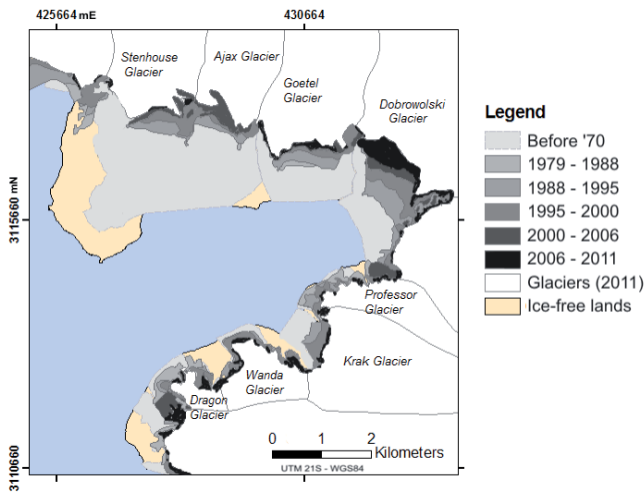
Figure 6 – Glacial retreat in the Martel Inlet. Glacier extend data were derived from lateral and bank morainal positions and orthophotomosaic (1979), SPOT (February of 1988; March of 1995 and 2000), Quickbird (October, 2006) and Cosmo-Skymed (February of 2011) orthorectified images.
