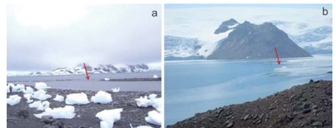
Figure 6 – Morainal banks in latest stability positions of the Wanda (a) and Dobrowolski (b) glaciers, Rosa Photo, 2013.
