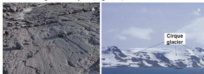
Figure 2 – Striated pavement in Wanda proglacial area (A) and glacial cirques in the Keller Peninsula (B). January, 2011.
