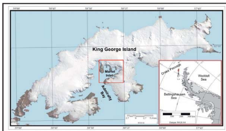
Figure 1 – Martel Inlet location in King George Island, Antarctica.
