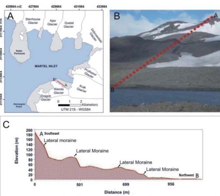
Figure 4 – Topographical profile A-B (dashed line – Figure B) shows morainic ridges in Wanda Glacier (Figure A) marginal area (Figure C).
